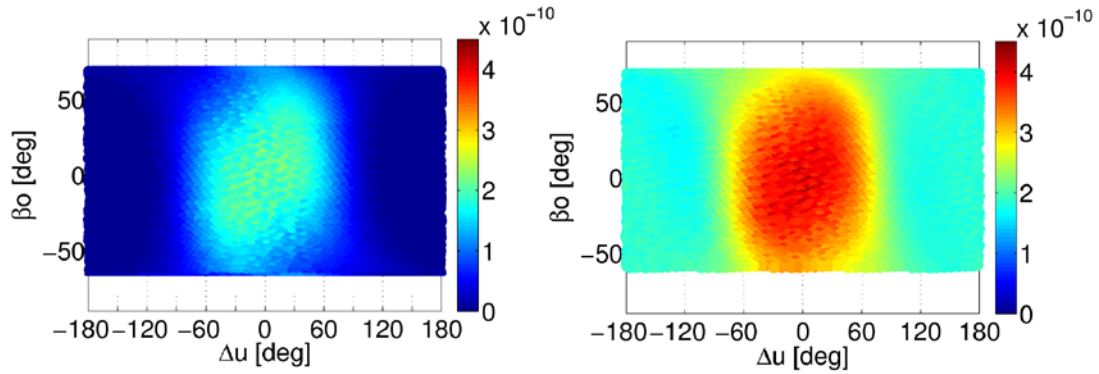
Figure 3. LAGEOS-2 acceleration due to reflectivity ( left ) and reflectivity + emissivity ( right ) for the radial direction where \beta_0 is the elevation angle of the Sun over orbital plane and \Delta u is argument of latitude w.r.t. the Sun (see Fig. 2 from Sośnica et al., 2014). Units: \text{m/s}^2 .
